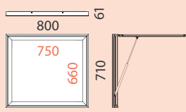
Ref. 4140-C2
