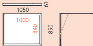
Ref. 4140-C
