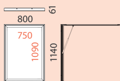
Ref. 4140-C1
